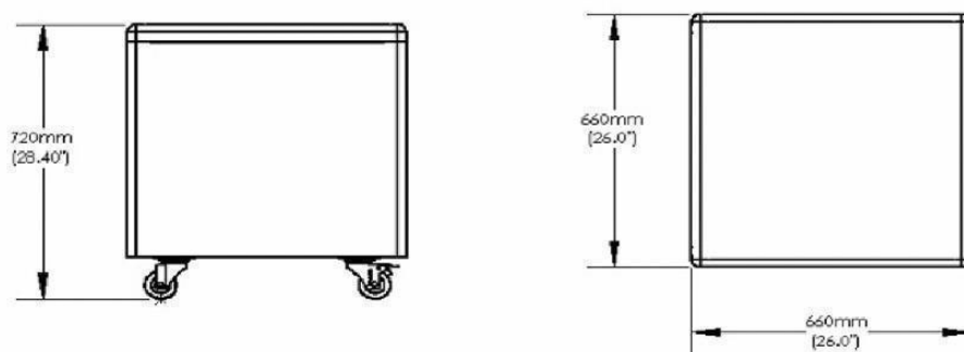
CUBICAL TYPE | 660 x 660 x 720 (in mm)
